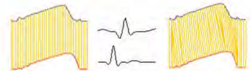
Figure 3. One to one alignment on time axis vs. non-linear alignment (warped time axis). Nonlinear curve alignment is important in pattern recognition of ECG signals. Wavelet analysis dose not allow this type of flexibility in pattern recognition and matching.
