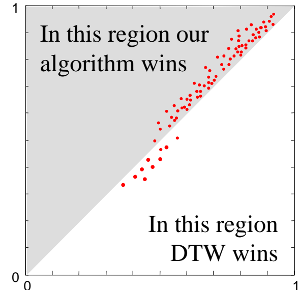
Figure 5. Each of our 100 motions plotted as a point in 2 dimensions. The X value is set to the distance to the nearest neighbor from the same class, and the Y value is set to the distance to the nearest neighbor from any other class.
