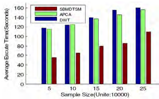
Figure 6. Average execute time
