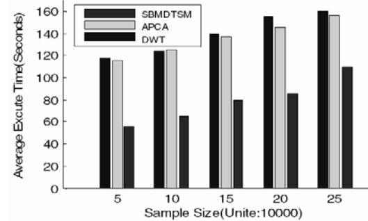
Figure 6. Average execute time
