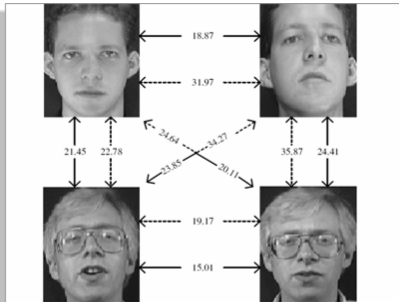
Figure 3. The distances of four faces by 2DDW and Euclidean norm. The 2DDW distances are shown on solid lines and Euclidean distances on dotted lines.
